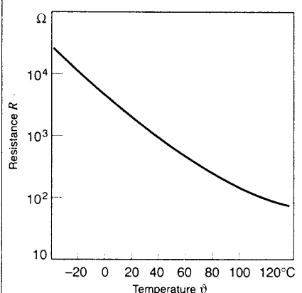
Characteristic curve 2
