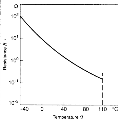
Characteristic curve 1
